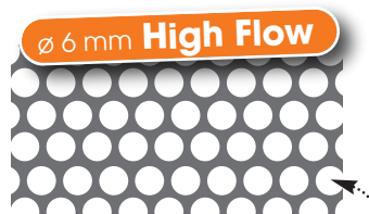
Free area 63%
